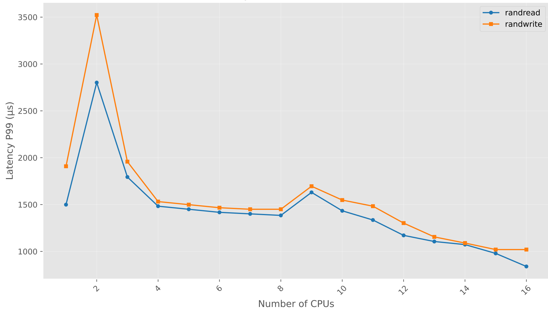
Latency P99 vs Number of CPUs
